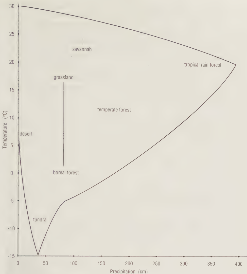
Figure 4.1 Biomes and climate
