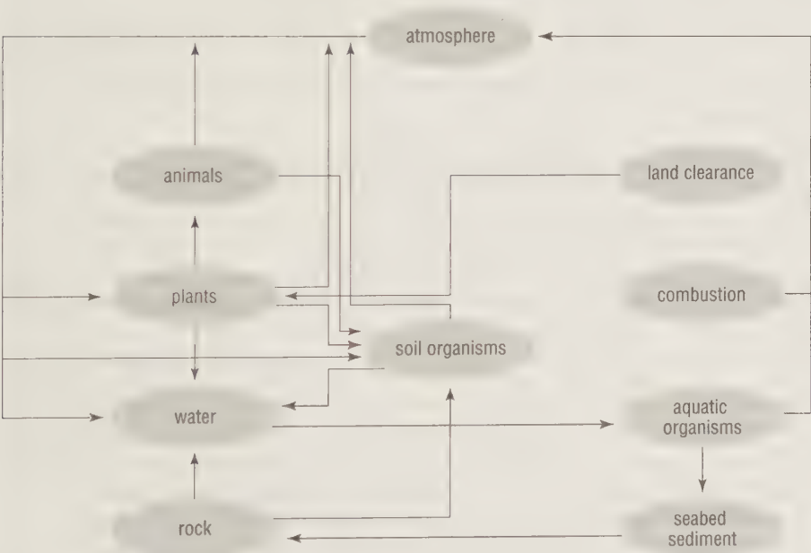
Figure 4.4 The carbon cycle
