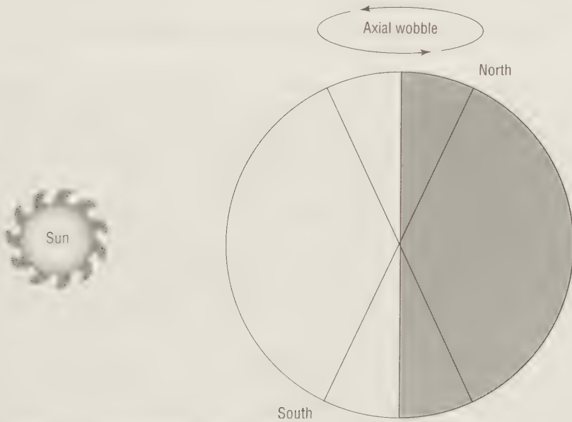
Figure 2.27 Wobble of the Earth's axis
