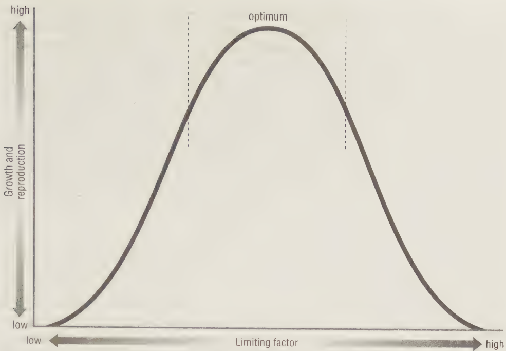
Figure 4.25 Limits of tolerance and optimum conditions
