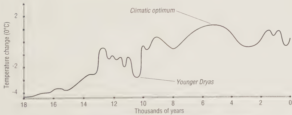
Figure 2.25 Temperature changes since the last glacial maximum (present temperature = 0)
