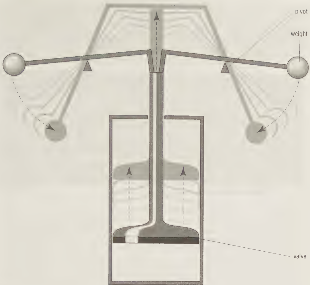
Figure 4.22 Speed governor of a steam engine
