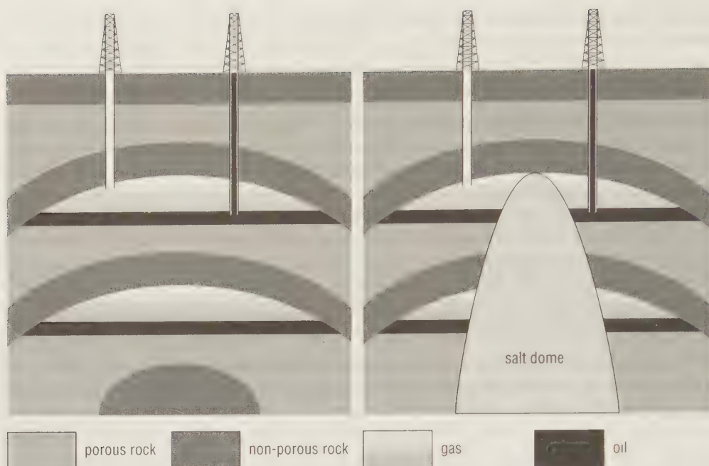
Figure 3.18 Structural oil and gas traps
