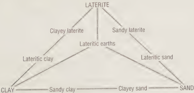
Figure 2.5 Gradation of clay and sand to laterite Source: Holmes, Arthur. 1965. Principles of Physical Geology . Nelson, Walton-on-Thames
