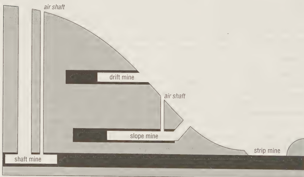
Figure 3.17 Types of coal mines
