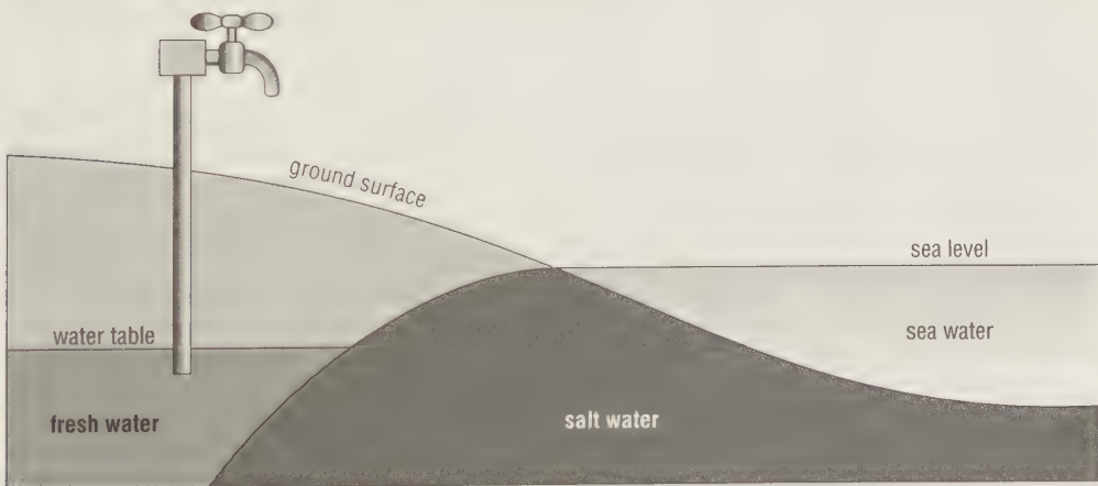
Figure 3.8 Salt water intrusion into a freshwater aquifer
