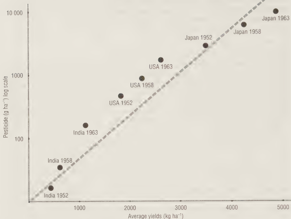
Figure 6.4 Pesticide use and crop yield
