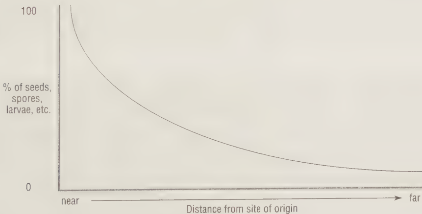
Figure 5.7 Common pattern for passive dispersal
